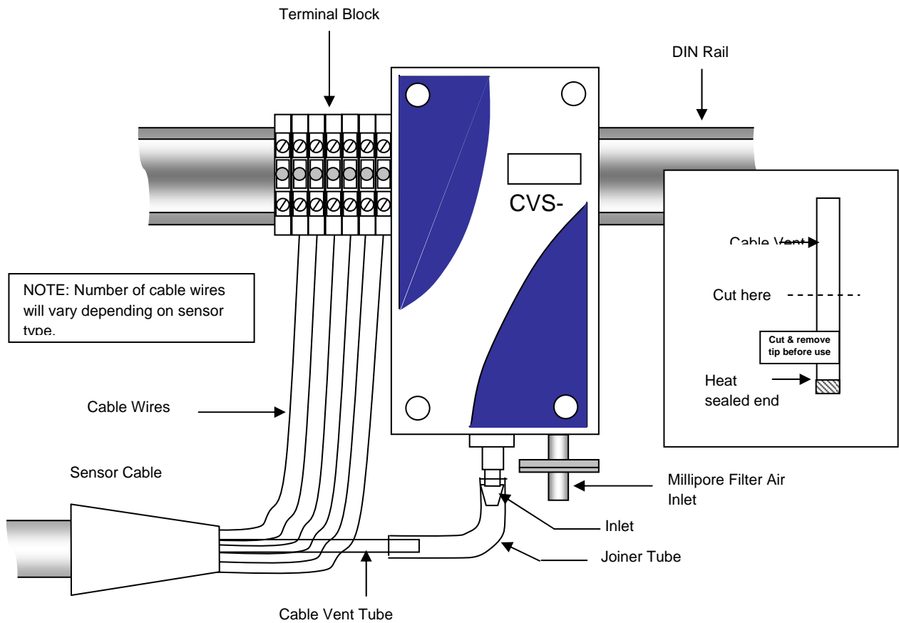
Figure 1. Single Installation, (Suggestion Only)
