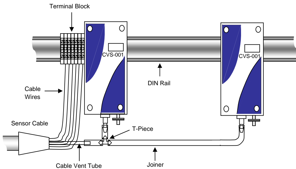
Figure 2. Multiple Units
